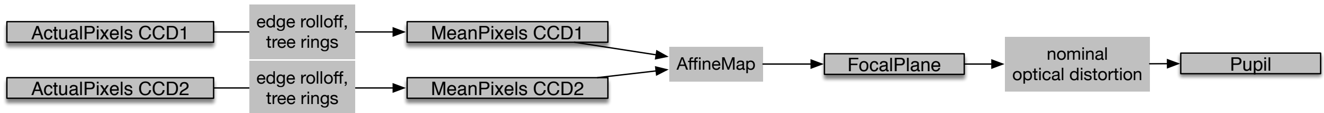
Example CameraGeom TransformGraph
